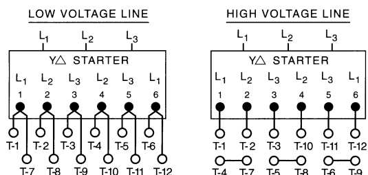
Dual Voltage, 12 Leads YΔ Start Connection
