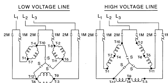
Dual Voltage, 12 Leads YΔ (Star-Delta) Start Connection
