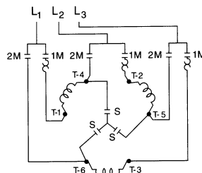
Single Voltage, 6 Leads YΔ (Star-Delta) Start Connection
