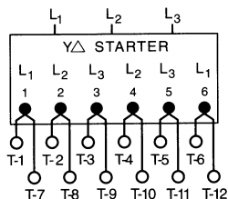
Single Voltage, 12 Leads YΔ Start Connection
