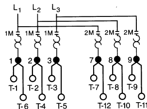
Single Voltage, 12 Leads Part Winding Start Connection
