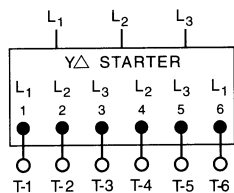
Single Voltage, 6 Leads YΔ Start Connection
